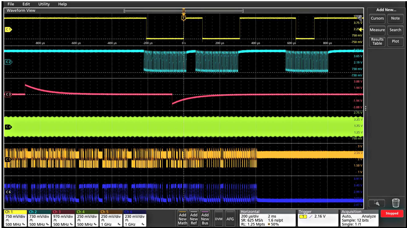
Figure 6: Stacked display mode enables easy visibility of all waveforms while maintaining maximum ADC resolution on each input for the most accurate measurements.
